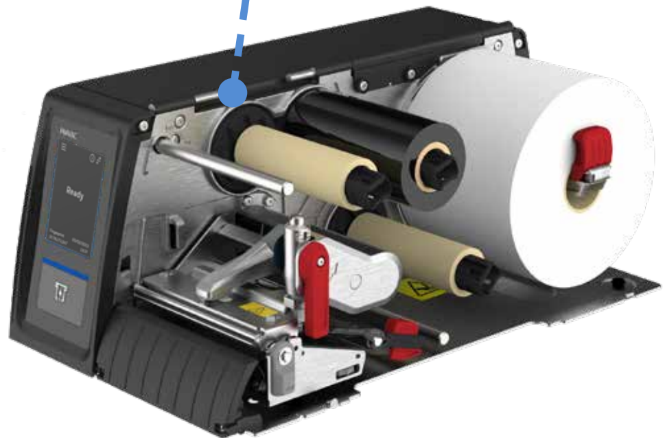
Ribbon Rewind - Empty Core Print Precision - Good Ribbon Removal - Good 100% Ribbon take up capacity from 220m ribbon.
