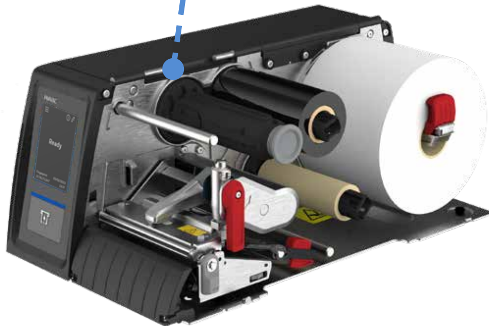
Ribbon Rewind - Small Collapsible Core Print Precision - Better Ribbon Removal - Better 80% Ribbon take up capacity from 220m ribbon.
