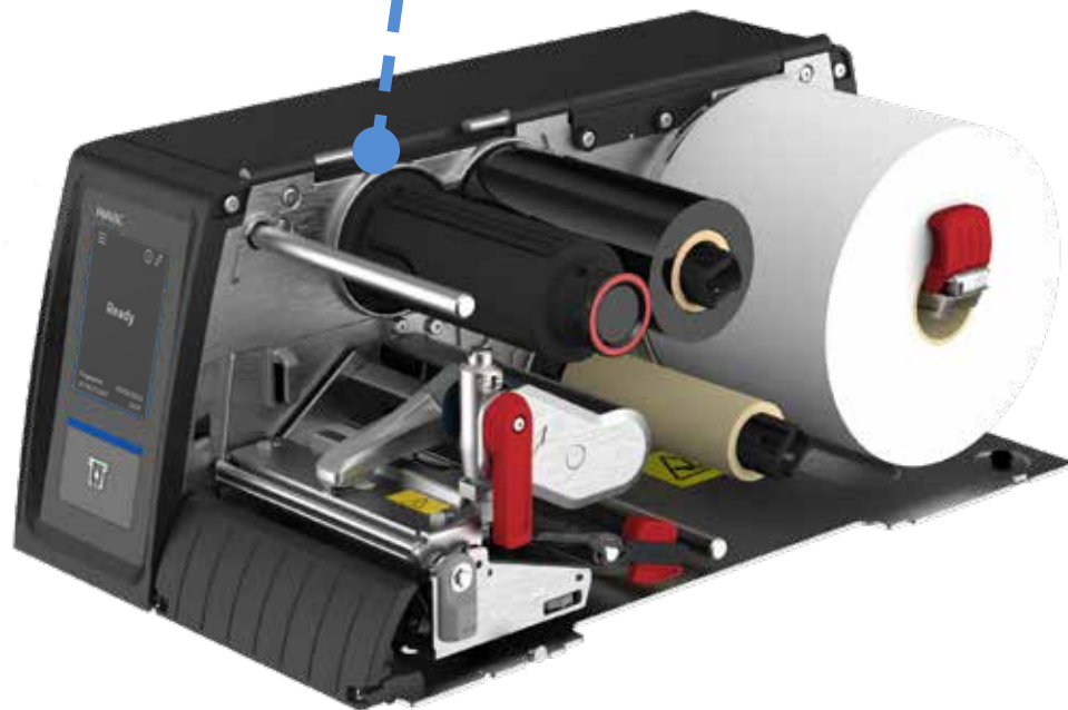
Ribbon Rewind - Large Collapsible Core Print Precision - Best Ribbon Removal - Best 50% Ribbon take up capacity from 220m ribbon.
